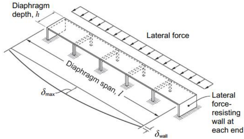
Figure 11. Effect of diaphragm deformations on distribution of displacements and forces
