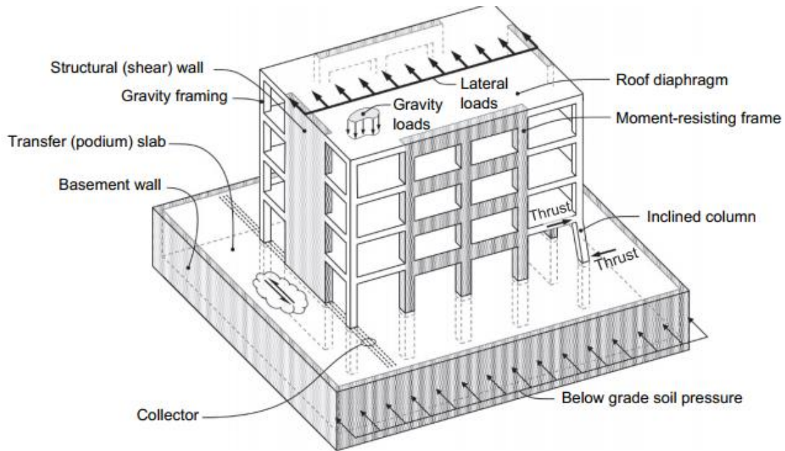
Figure 2. Role of diaphragms.
