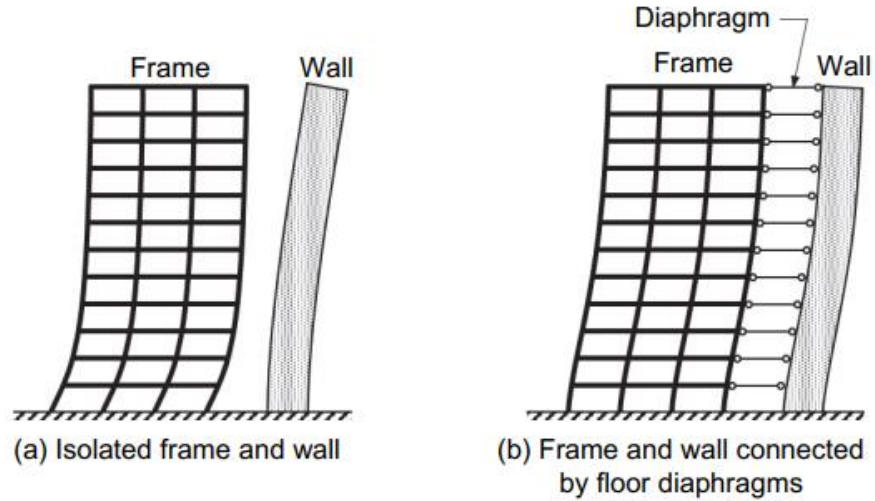
Figure 8. Diaphragms develop transfer forces by imposing displacement compatibility between different vertical elements of the seismic force-resisting system.
