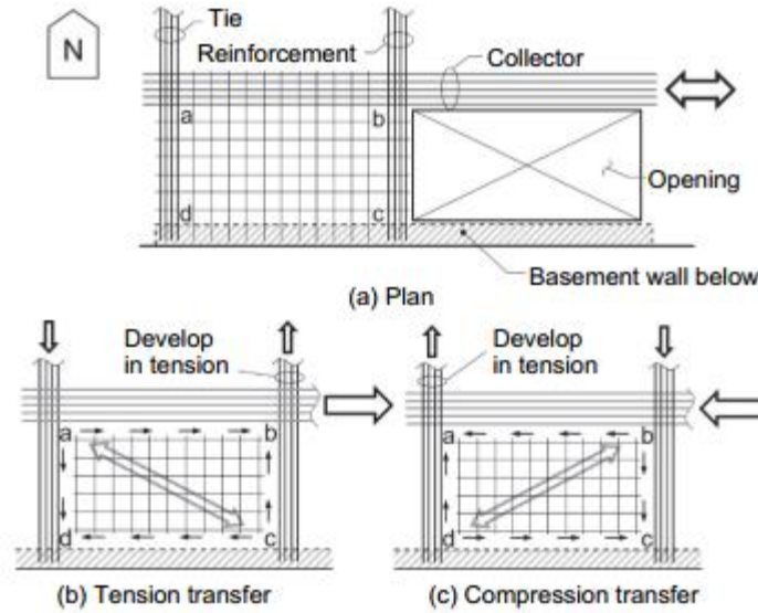
Figure 25. Reinforcement to transfer collector force around an opening.
