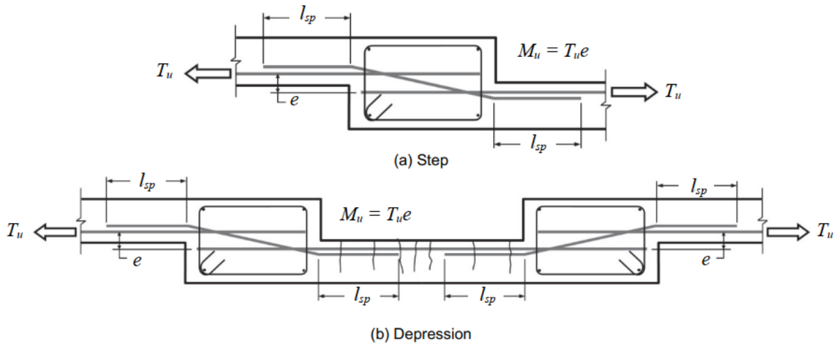
Figure 27. Collector reinforcement passing through a step and depression
