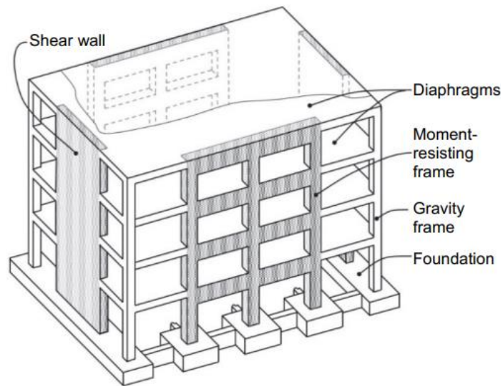
Figure 1. Isometric view of a basic building structural system comprising horizontal elements (diaphragms), vertical elements (walls and frames), and foundation.
