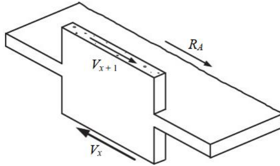
Figure 10. Force R_A transferred between diaphragm and wall can be obtained by section cuts through wall.
