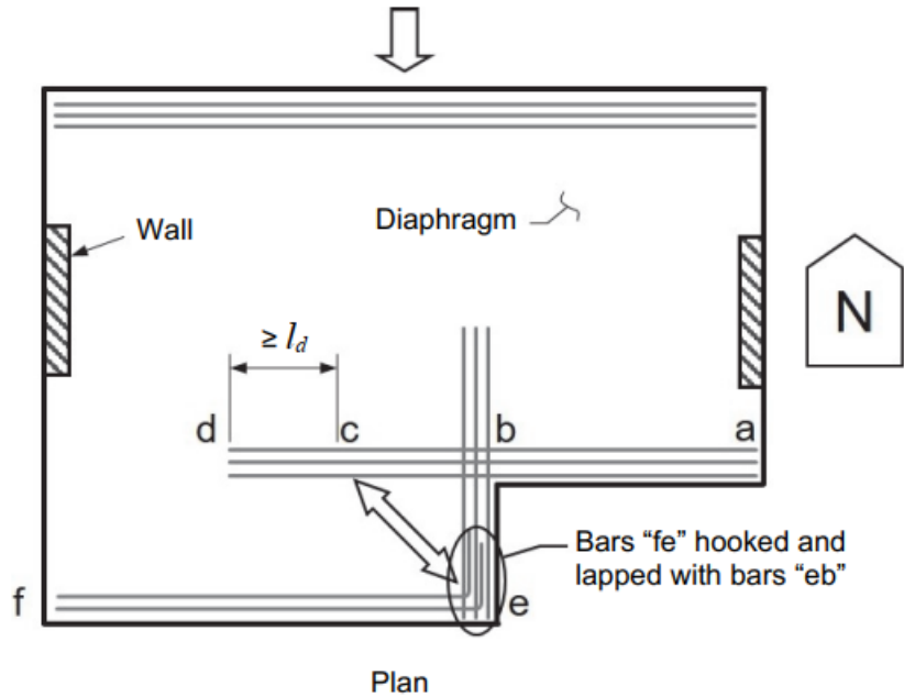
Figure 26. Reinforcement associated with re-entrant corners
