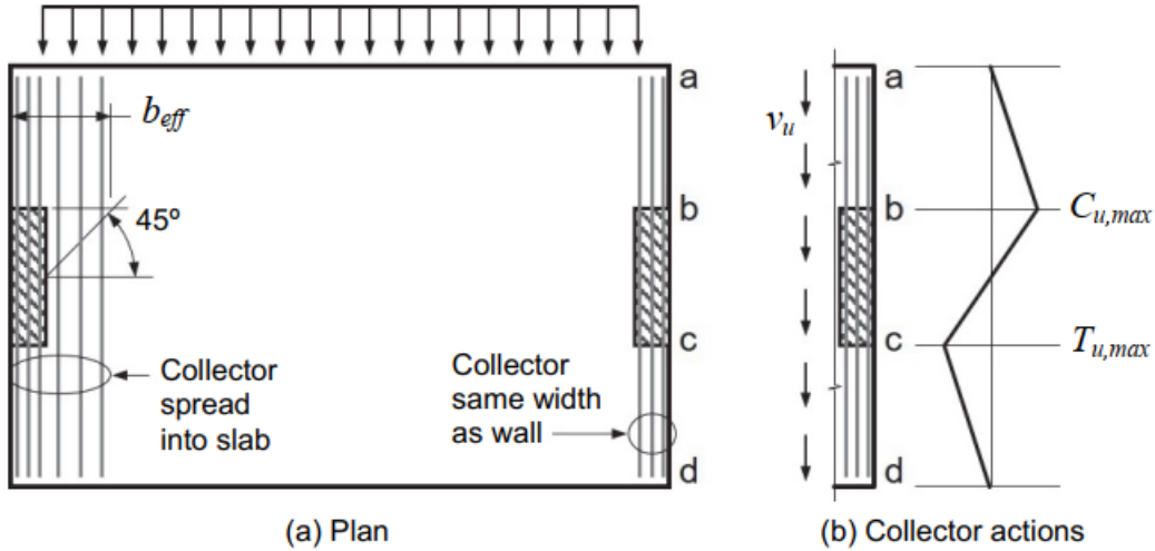
Figure 4. Collectors
