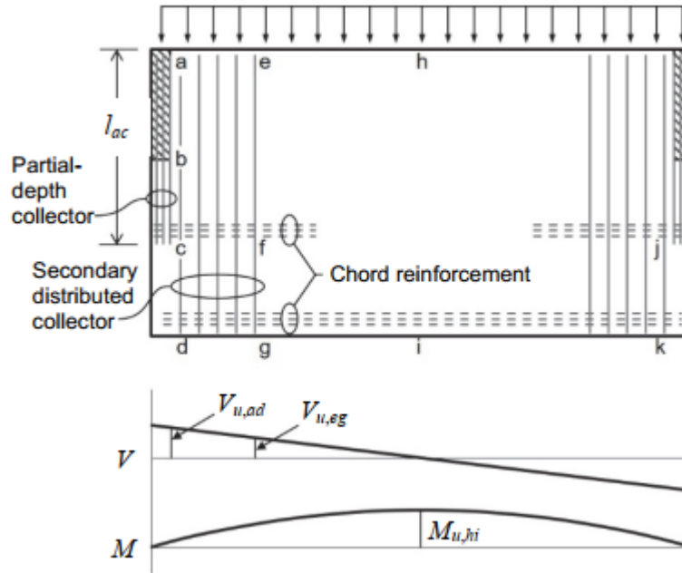
Figure 19. Partial-depth collector
