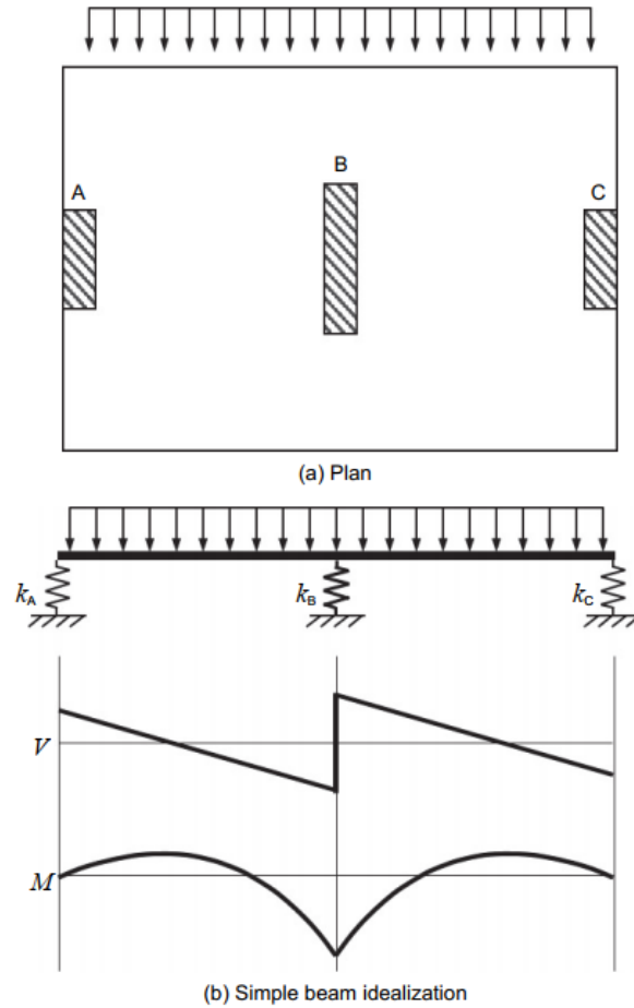
Figure 12. Equivalent beam-on-springs model
