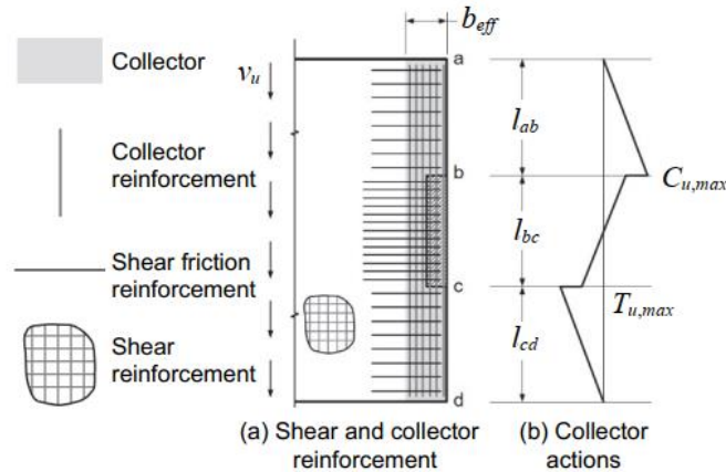
Figure 23. Shear reinforcement, collector reinforcement, and shear friction reinforcement.
