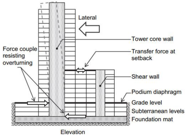
Figure 9. Diaphragm transfer forces at irregularities in the vertical elements of the seismic force-resisting system
