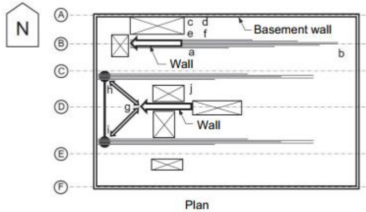
Figure 16. Challenging design conditions
