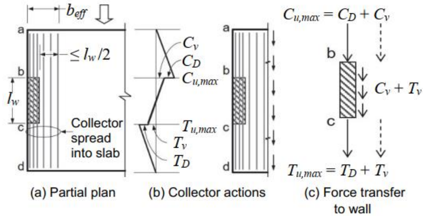
Figure 14. Force transfer where a collector is wider than the vertical element to which it transmits diaphragm shears.
