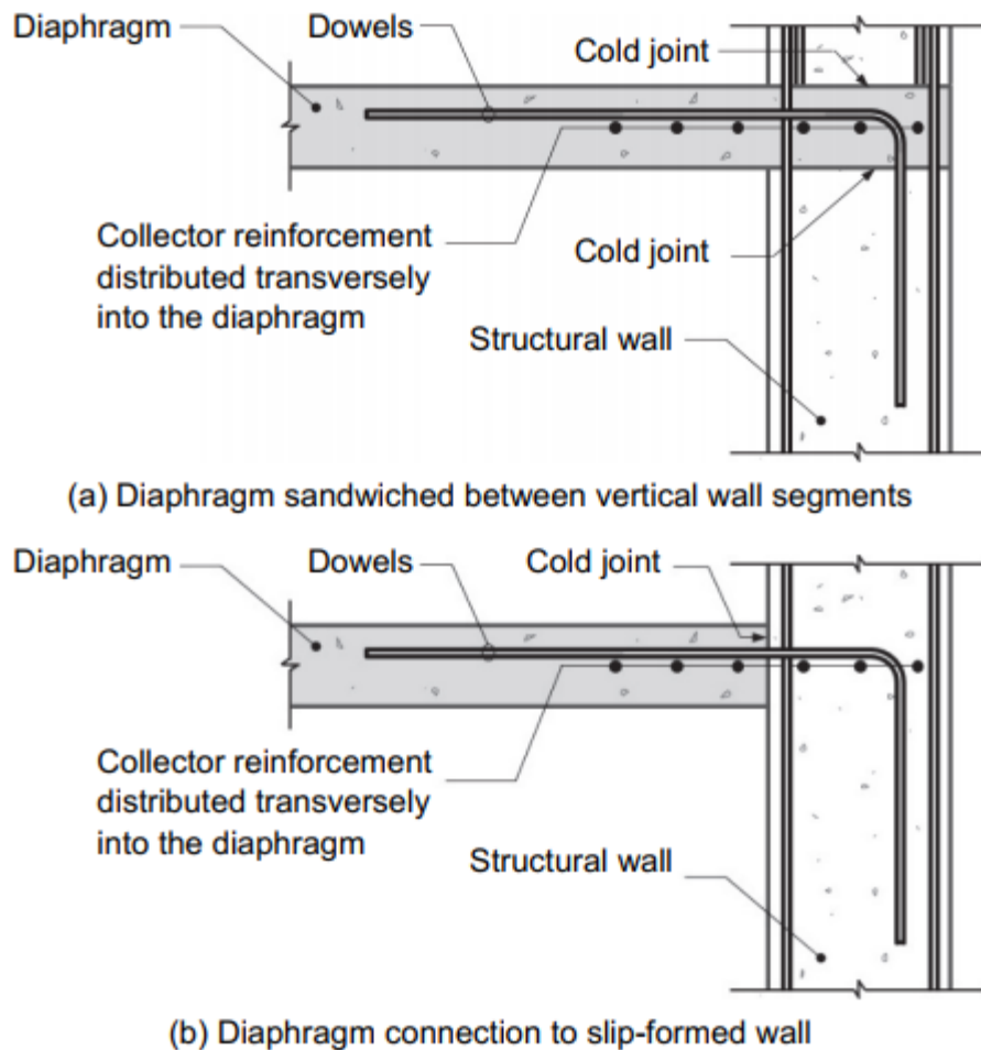
Figure 24. Shear reinforcement, collector reinforcement, and shear friction reinforcement.
