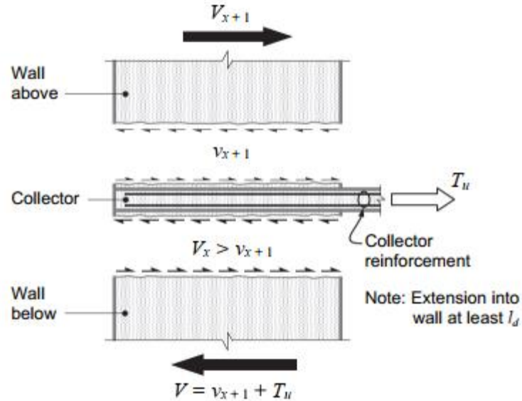
Figure 20. collector force directly to shear wall
