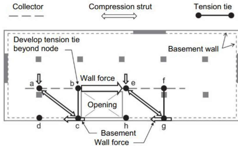
Figure 15. Strut-and-tie model at force transfer to basement wall
