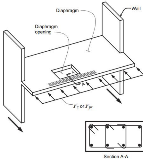
Figure 22. Confinement reinforcement in axial struts around openings.
