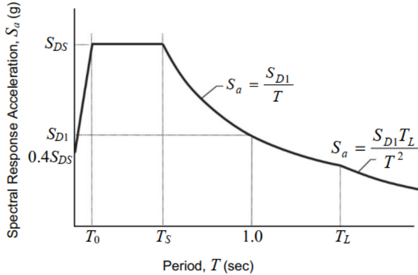
Figure 6. ASCE 7 design response spectrum showing spectral response acceleration as a function of vibration period.
