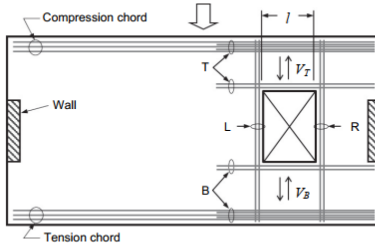
Figure 18. Diaphragms with large openings.
