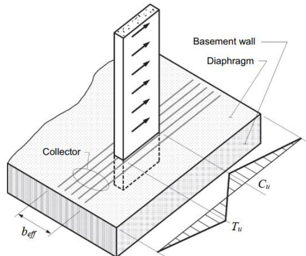
Figure 5. Collector transferring shear from the wall into the podium diaphragm
