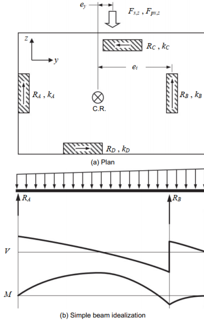
Figure 13. Corrected equivalent beam model
