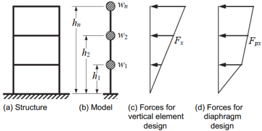
Figure 7. Design forces for vertical elements and diaphragms.
