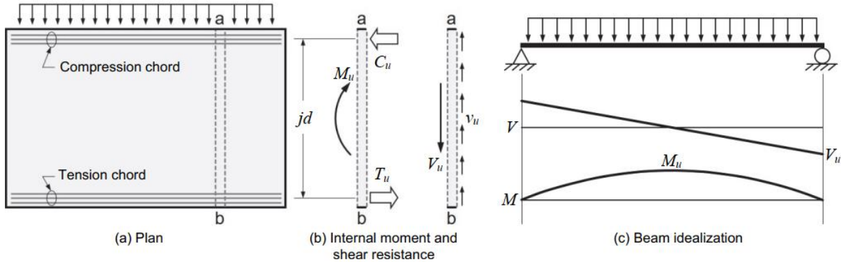
Figure 3. Moment and shear at a section cut
