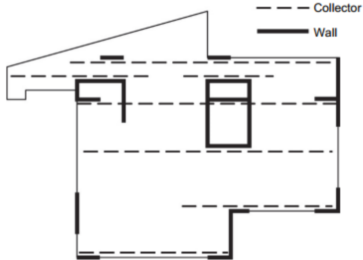
Figure 17. Irregularly shaped diaphragm
