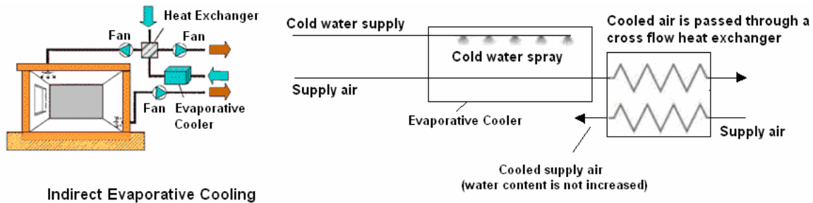
Indirect Evaporative Cooling
