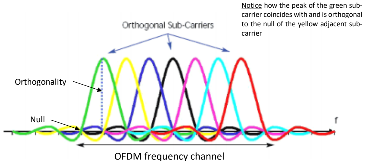
Figure 4. OFDM Orthogonality
